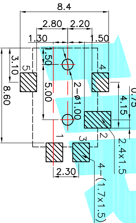
P.C.B LAYOUT(Copper-side view)
