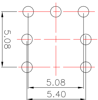
PCBLayout(Pattern Side)
